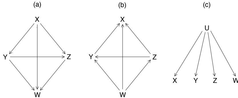
Figure 9. Two complete path diagrams, and a factor analysis model, all having the same covariance matrix.
