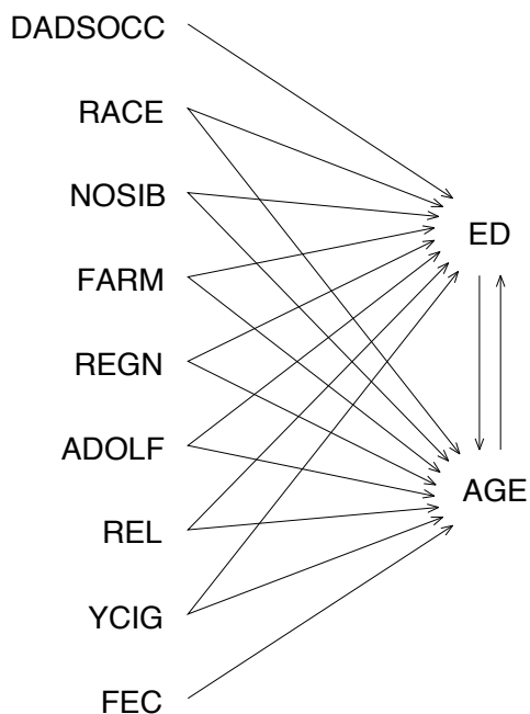
Figure 3. The model in diagram form (Rindfuss et al. 1980; SGS p. 140; CG p. 15). Variables are defined in Table 2 below. Explanatory variables (DADSOCC, RACE, etc.) are correlated; error terms are not shown in the diagram.
