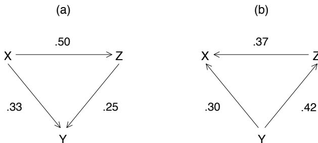
Figure 8. Graphs (a) and (b) have the same covariance matrix. Both are complete: there is an arrow from every variable to every other variable. The numbers on the arrows are path coefficients, that is, standardized regression coefficients.
