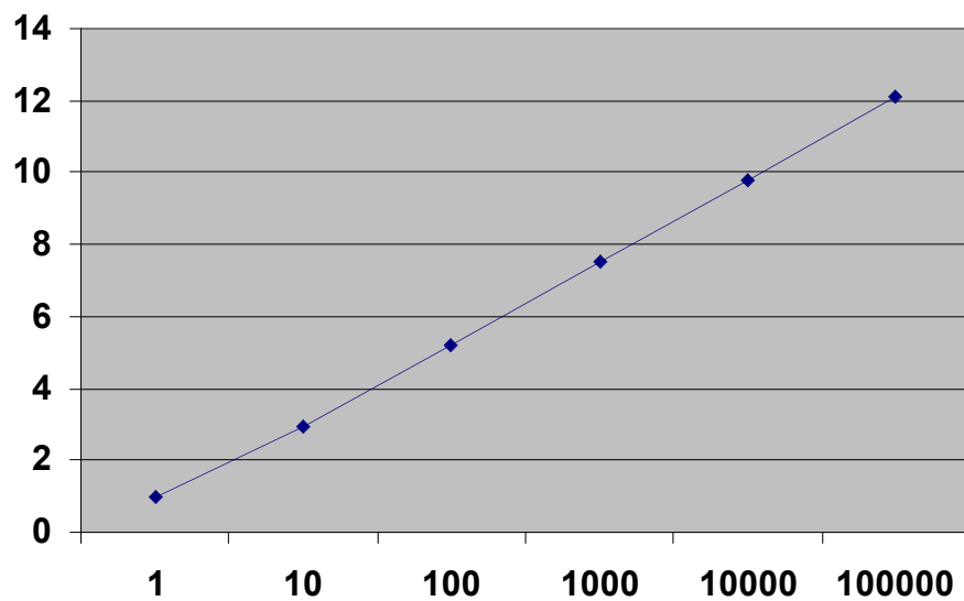
Figure 1: Expected Number of Categories
