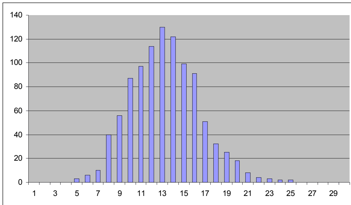
Figure 5: Number of Signals after 100,000 iterations of reinforcement with invention. Frequency in 1000 trials.
