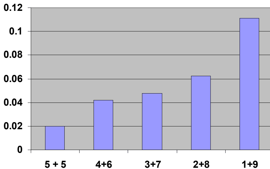
Figure 2: Probability of Partitions of 10 into two categories.
