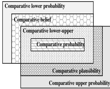
Figure 2: Relationships among the classes of ordinal relations.
